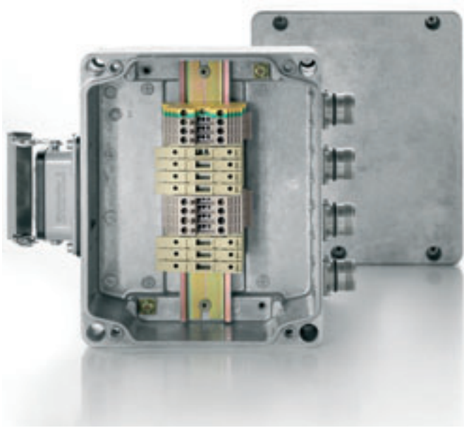
Assembled enclosures, with terminal strips and connectors
