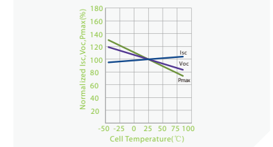
Temperature Dependence of Isc, Voc, Pmax
