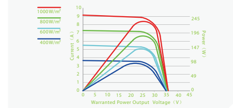
Current-Voltage and Power-Voltage Curves (245W)
