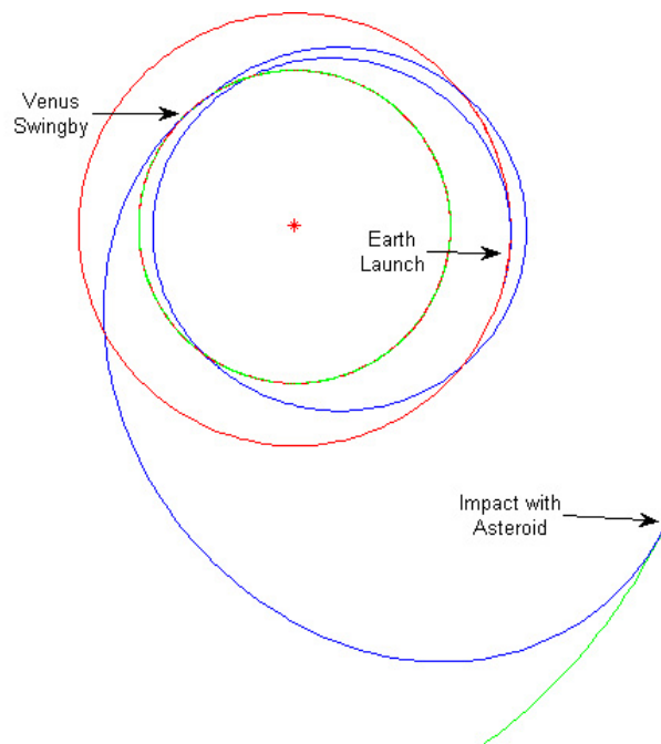
Figure 3.13: Earth-Venus-Asteroid trajectory
