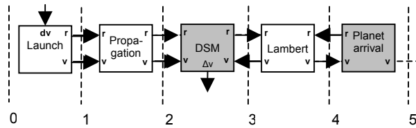
Fig. 1.21. Sections at which the states shall be defined.
