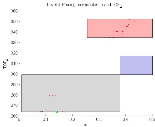
Fig. 2.32. Level 4 pruned space: variables \alpha and TOF. The green point is the BepiColombo solution.
