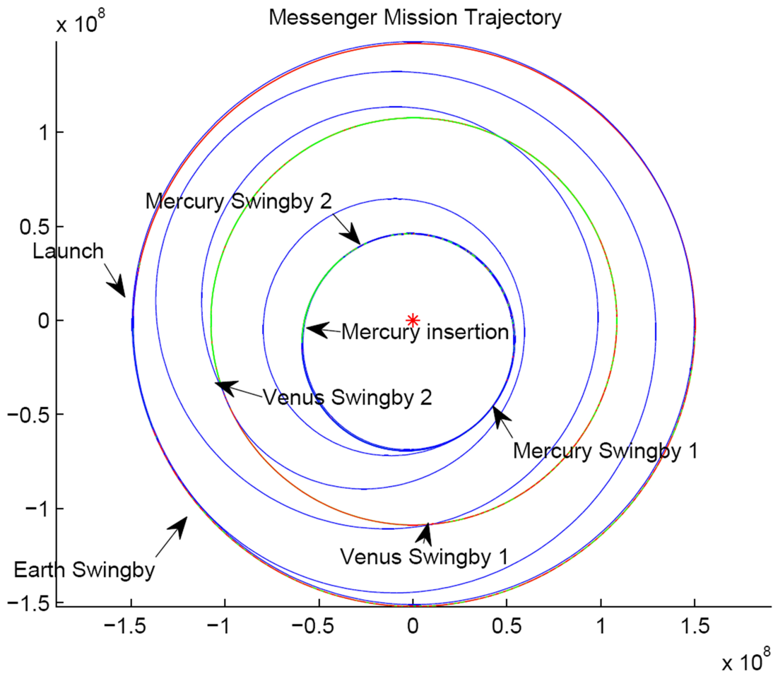
Figure 3.7: Optimised MESSENGER Trajectory
