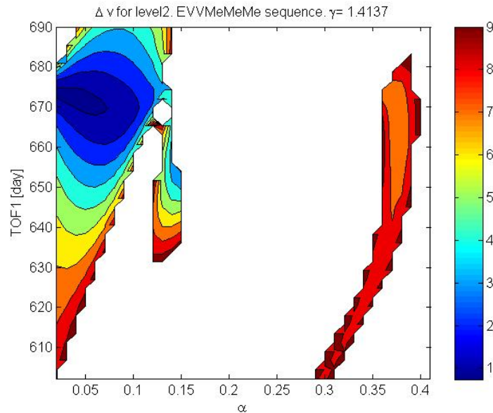
Fig. 2.39. \Delta v at level 2 for different TOFs and angle \alpha
