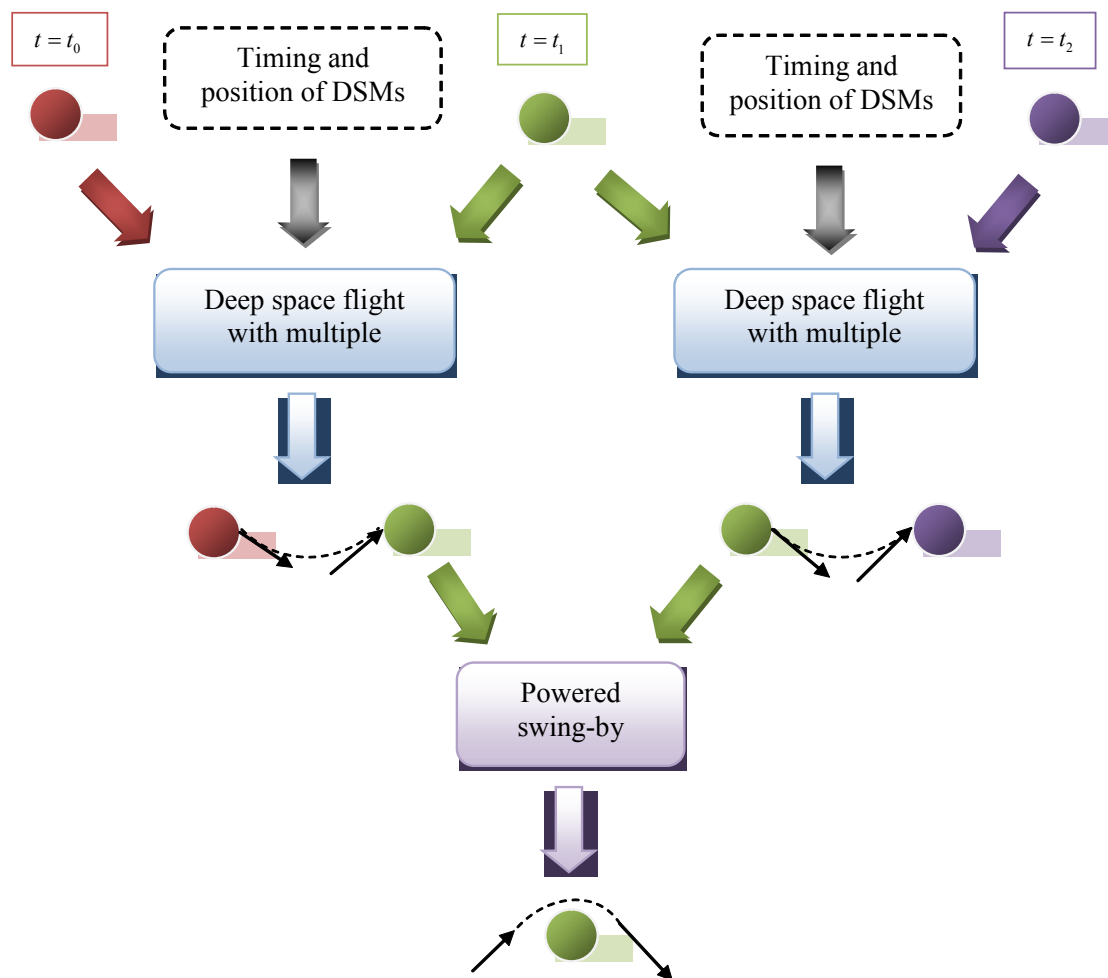
Fig. 1.10. This schema represents the procedure to build a trajectory using model 2. After having fixed the times at the planets, it is possible to compute the deep space flight phases, given the parameters. Then two consecutive deep space flight phases can be joined together through the swing-by.
