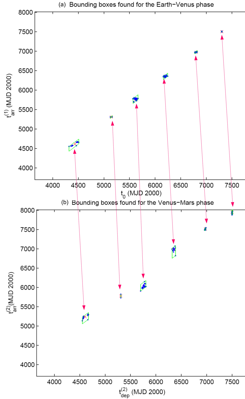
Figure 3.3: (a) Illustration on the located bounding boxes on the t_0 - t_{\text{arr}}^{(1)} plane for the estimates of the feasible regions for the Earth-Venus phase. The actual bounding boxes are in six dimensions. (b) Projection on the t_{\text{dep}}^{(2)} - t_{\text{arr}}^{(2)} plane of the located bounding boxes for the estimates of the feasible regions for the Venus-Mars phase. The actual bounding boxes are in six dimensions. The double headed arrows show the six solution families that were identified.
