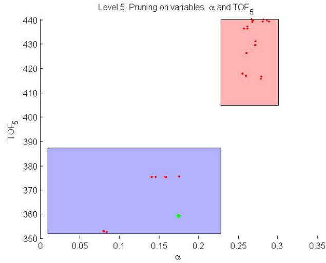
Fig. 2.30. Level 5 pruned space: variables \alpha and TOF. The green point is the BepiColombo solution.
