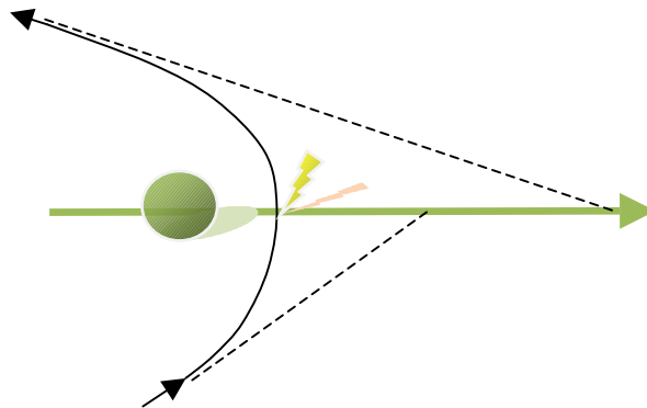
Fig. 1.9. Schematic representation of the powered swing-by. The propelled, instantaneous manoeuvre is performed at the pericentre of the two hyperbolae.
