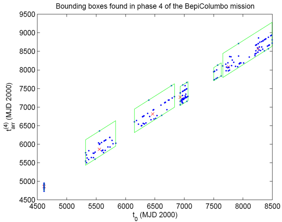
Figure 3.9: Projection on the t_{\text{dep}}^{(4)} - t_{\text{arr}}^{(4)} plane of the located bounding boxes for the estimates of the feasible regions for phase 4 of the BepiColombo mission. The actual bounding boxes are in six dimensions
