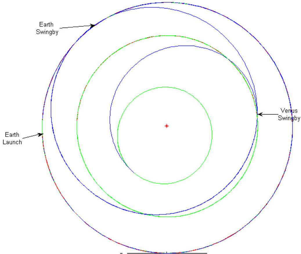
Figure 3.11: Earth-Earth-Venus-Mercury trajectory
