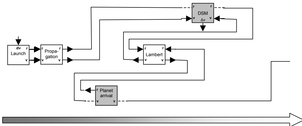
Fig. 1.22. Blocks for the sequence in Fig. 1.21 positioned along a horizontal axis according to their evaluation order.
