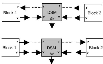
Fig. 1.15. Two possible feasible sequences of blocks.
