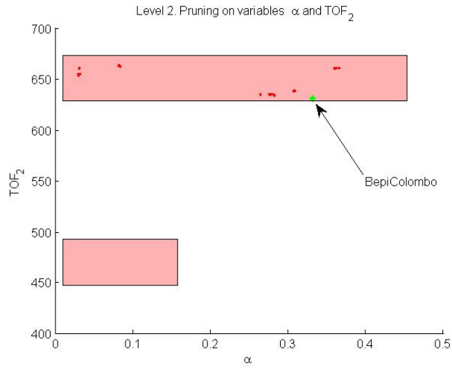
Fig. 2.36. Level 2 pruned space: variables \alpha and TOF_2 . The green point is the BepiColombo solution.
