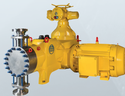
The Primeroyal X with metallic liquid end and PTFE (Teflon®) double diaphragm, horizontal motor configuration, and actuator with integrated electronics.
