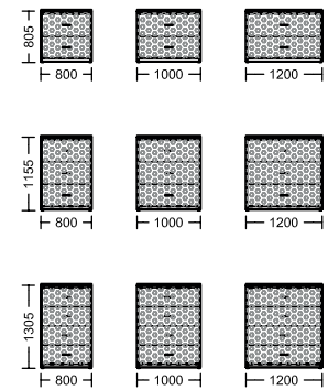
basic element / drawer cabinets with handle
