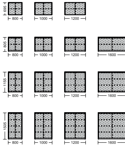
basic element / sliding door cabinets / acoustically absorptive
