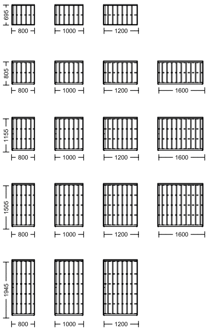
basic element / horizontal roller shutter cabinets
