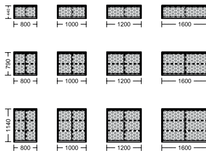
additional element / sliding door cabinets / acoustically absorptive
