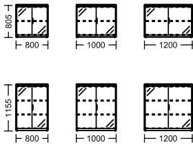
basic element / folding door cabinets GLASS with handle
