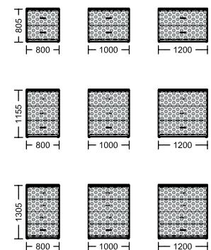
basic element / drawer cabinets with handle / acoustically absorptive
