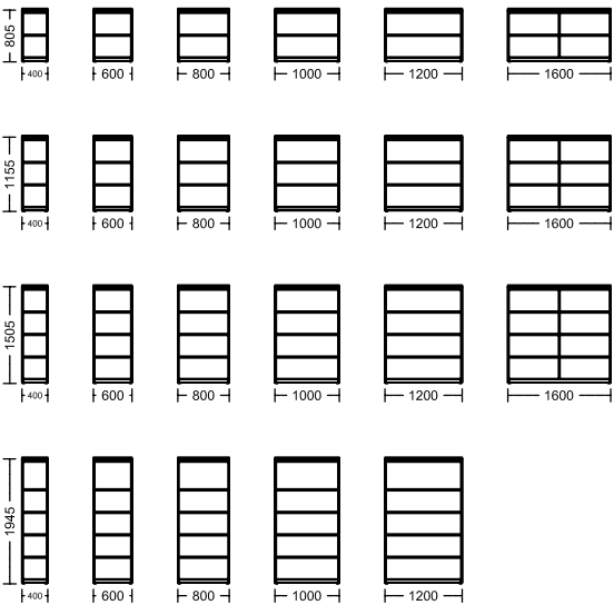
basic element / open cabinets
