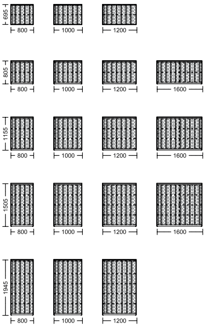
basic element / horizontal roller shutter cabinets / acoustically absorptive
