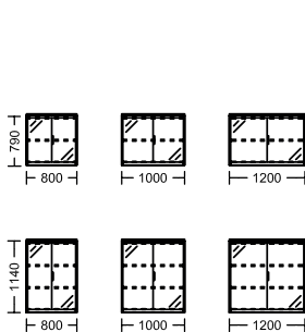
additional element / folding door cabinets GLASS with handle
