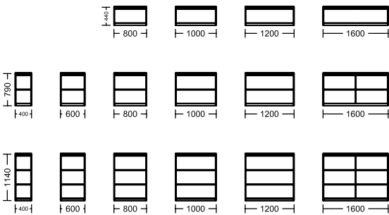
additional element / open cabinets
