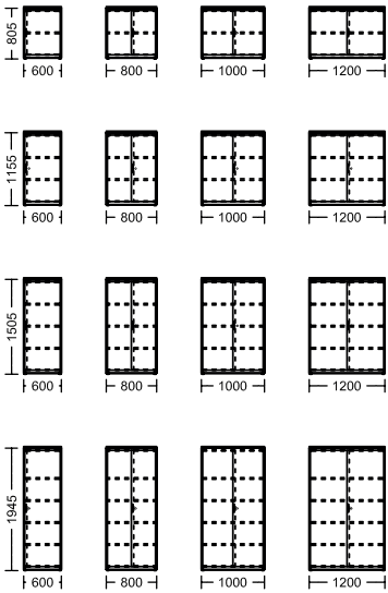
basic element / folding door cabinets with handle
