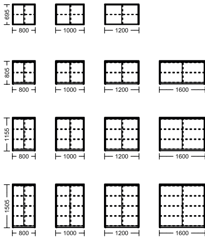
basic element / sliding door cabinets
