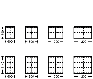
additional element / folding door cabinets with handle
