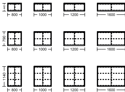
additional element / sliding door cabinets
