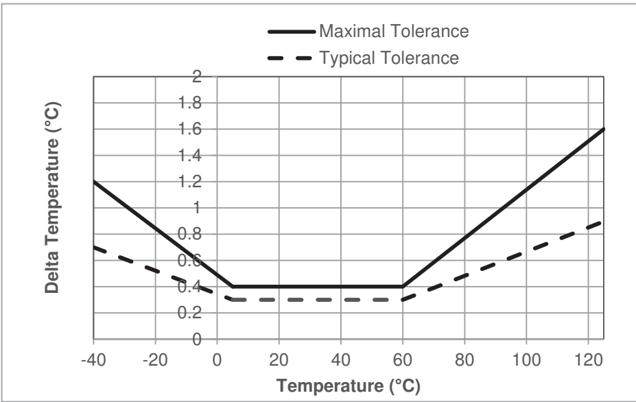
GRAPH 2 : TEMPERATURE ERROR BUDGET
