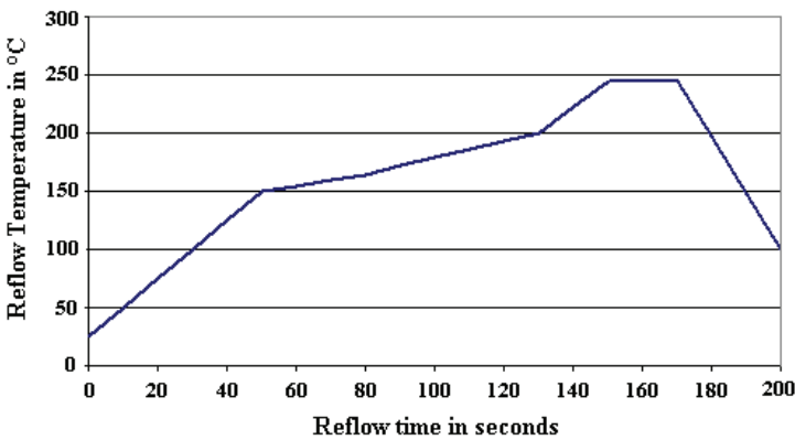
Lead Free Suggested Reflow Profile
