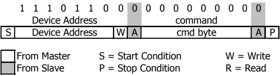
Figure 8: I 2 C ADC read sequence
