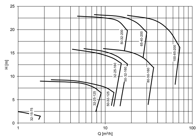
1800 rpm/60 Hz
