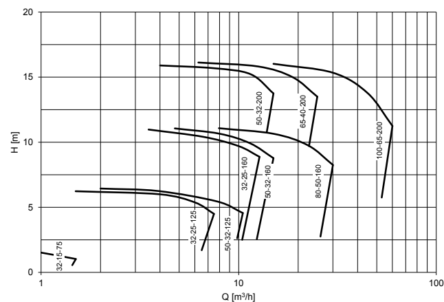
1500 rpm/50 Hz
