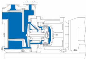
Close-coupled MKPL-S with baseplate -20°C to +150°C
