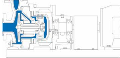
Frame-mounted MKPL with baseplate -20°C to +200°C
