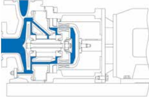
Close-coupled MKPL with baseplate -20°C to +200°C
