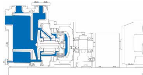
Frame-mounted MKPL-S with baseplate -20°C to +150°C
