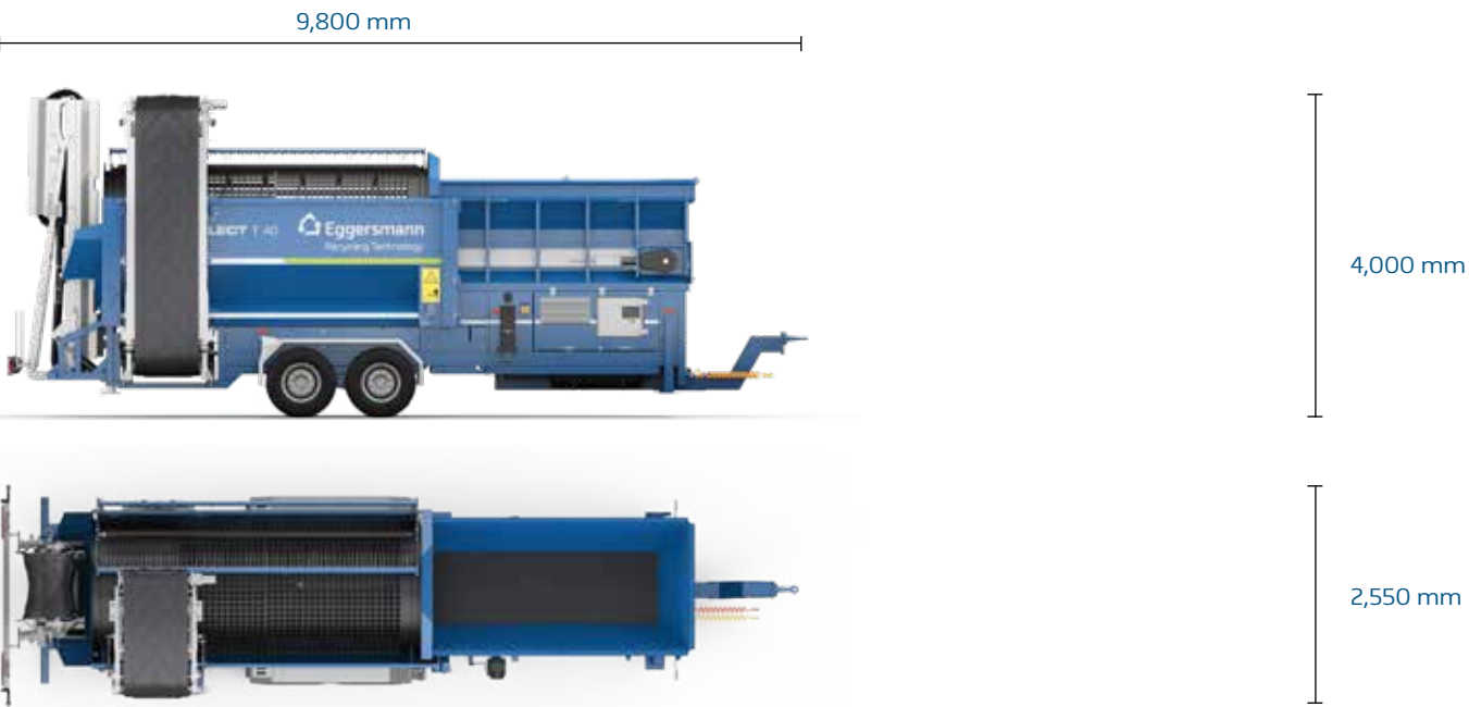
Transport position
