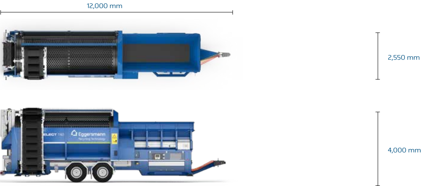
Transport position
