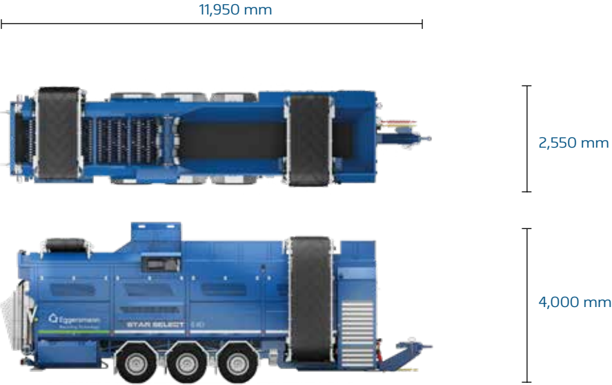
Transport position
