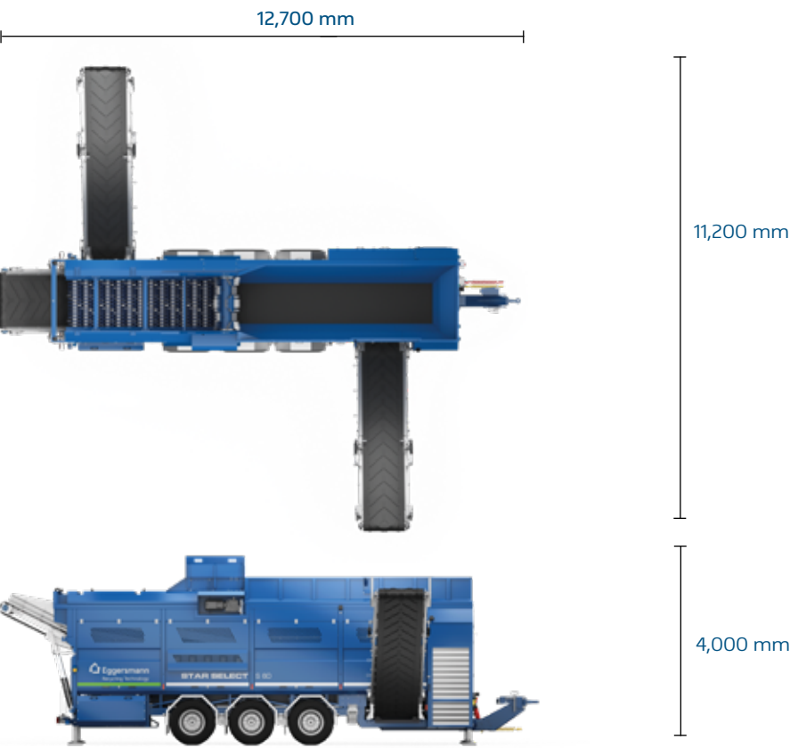
Working position
